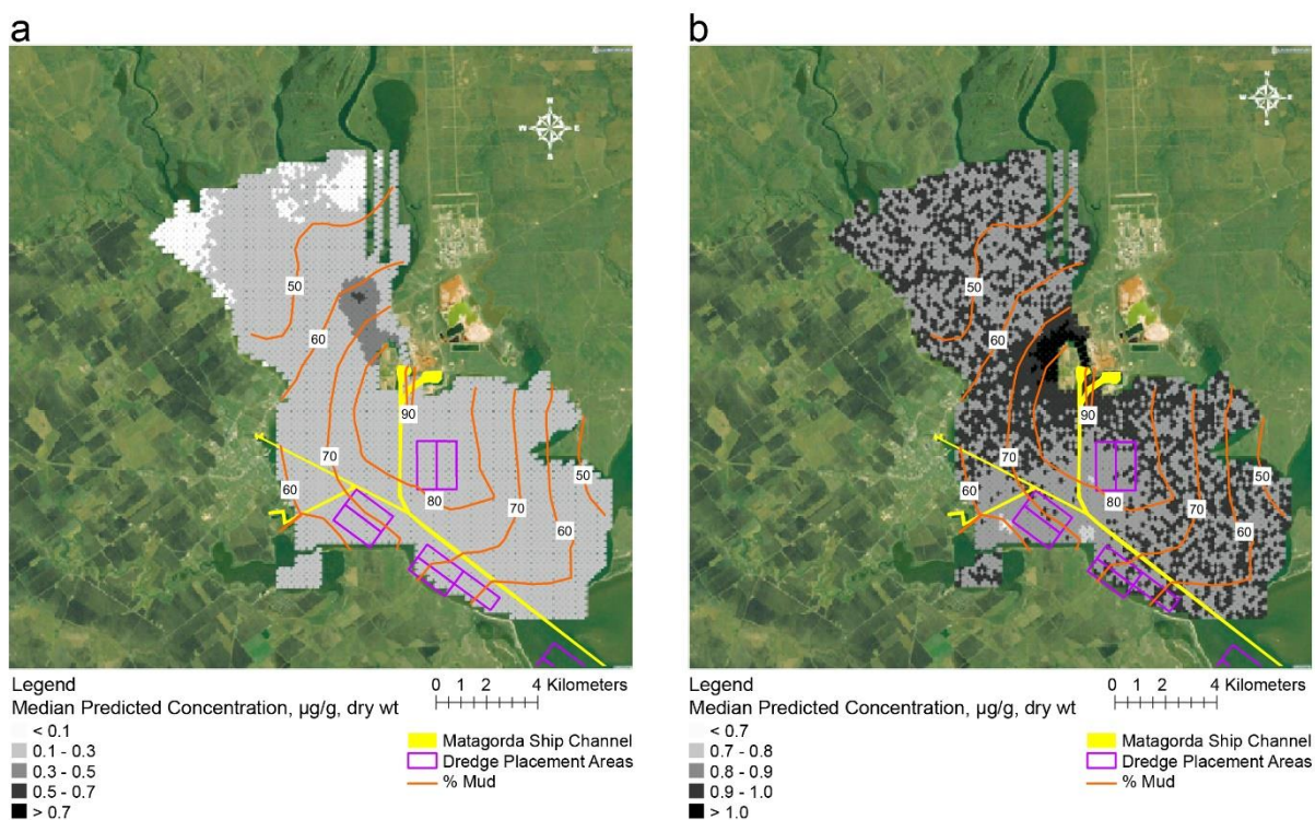
Figure 13. Mercury concentrations in Lavaca Bay (a) sediments, and oyster tissue (b) (Bissett et al. 2008), project location and footprint (Maglio 2021), and sediment grain size as percent mud in orange isopleths (White et al. 1989).
